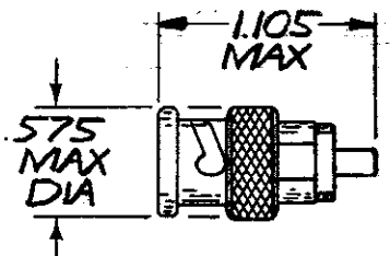
ASSEMBLED VIEW
