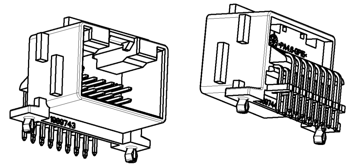
PERSPECTIVE VIEWS SCALE 2:1
