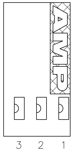
CAVITY NUMBER
