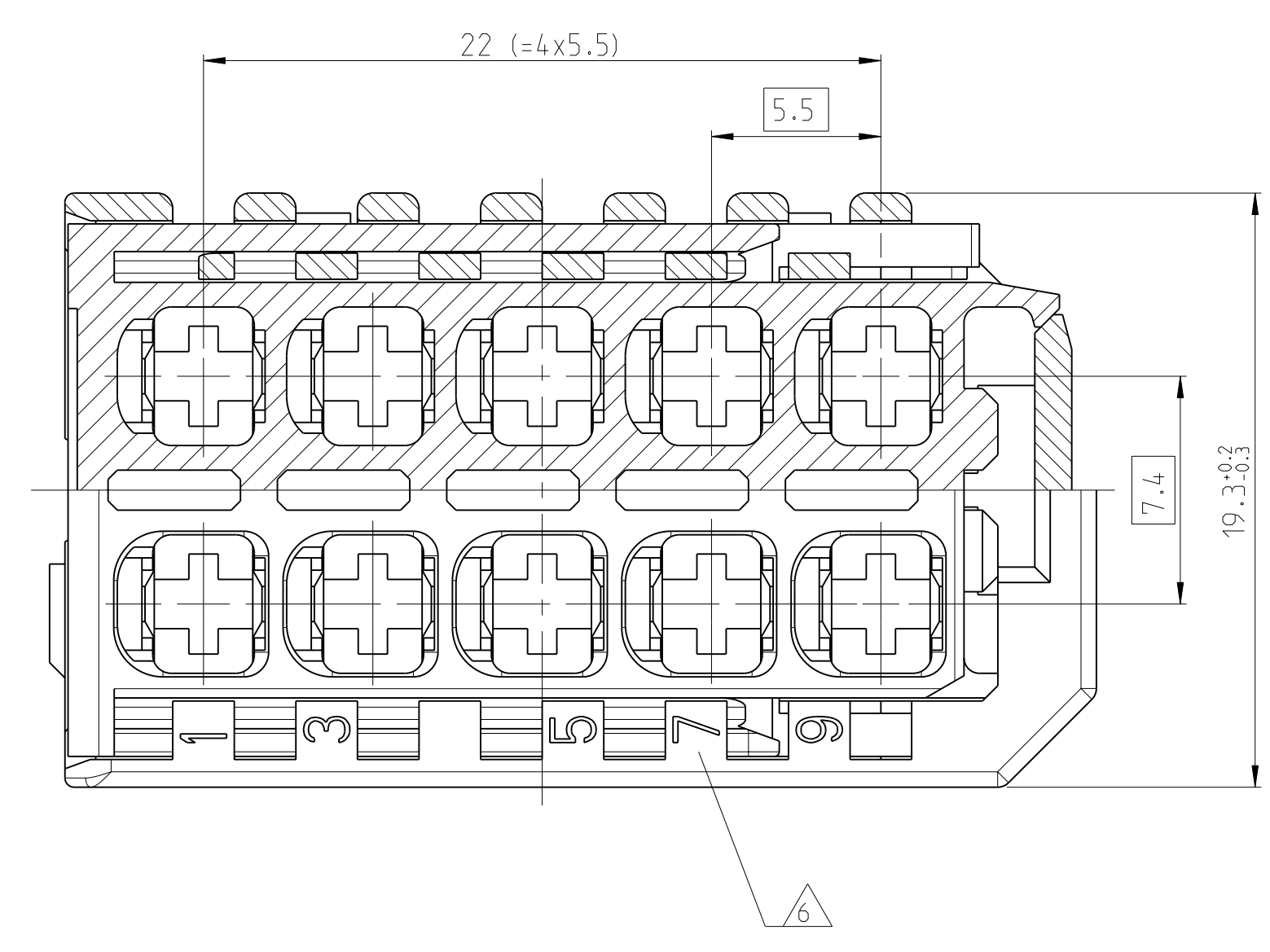
HOUSING IN PRE-LOCKED POSITION (DELIVERY CONDITION) Gehäuse in Vorraststellung (Lieferzustand)
