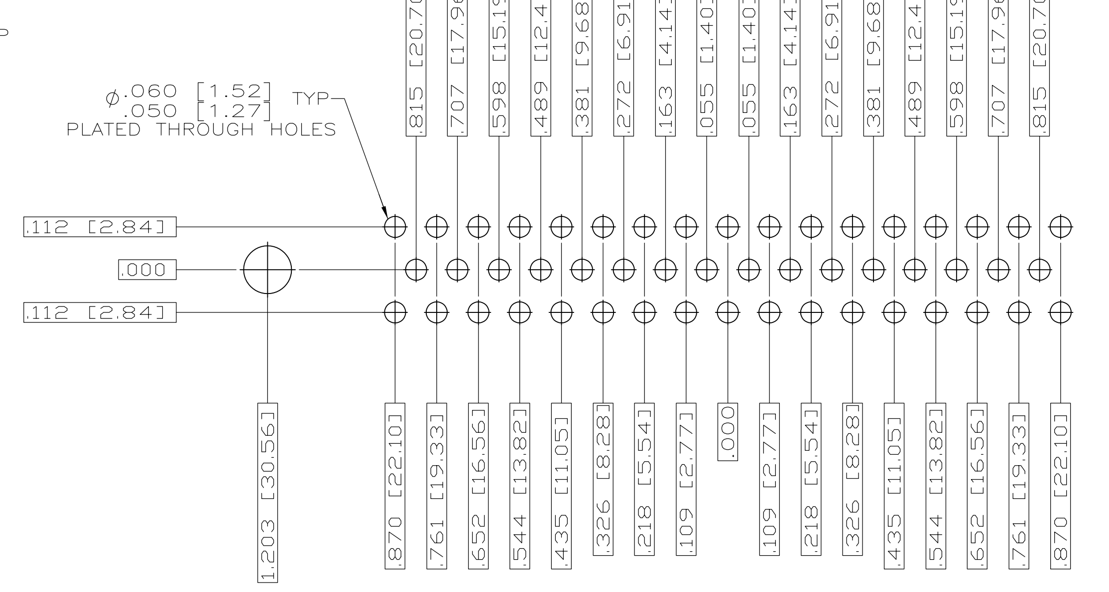
RECOMMENDED P.C. BOARD LAYOUT SHELL SIZE 5 (50 POSITION) ⚠
