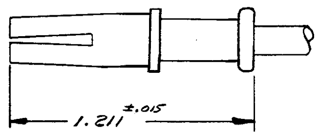
ASSEMBLED VIEW
