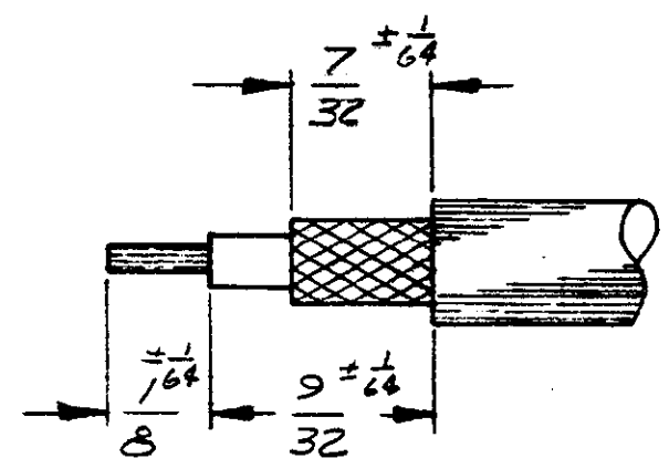
STRIP LENGTH
