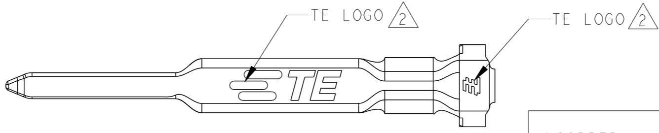
SECTION M-M
