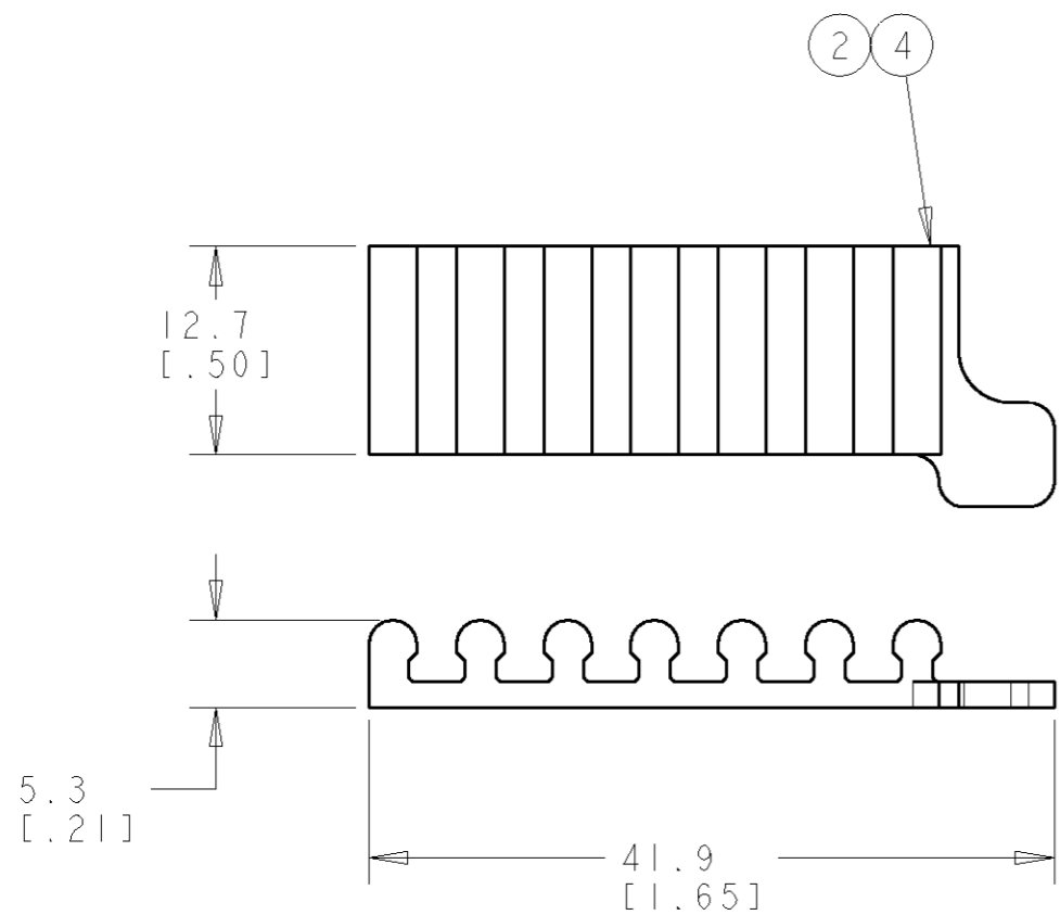
RIBBON FIBER CAP
