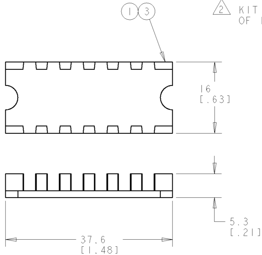
3MM JACKETED CABLE CAP
