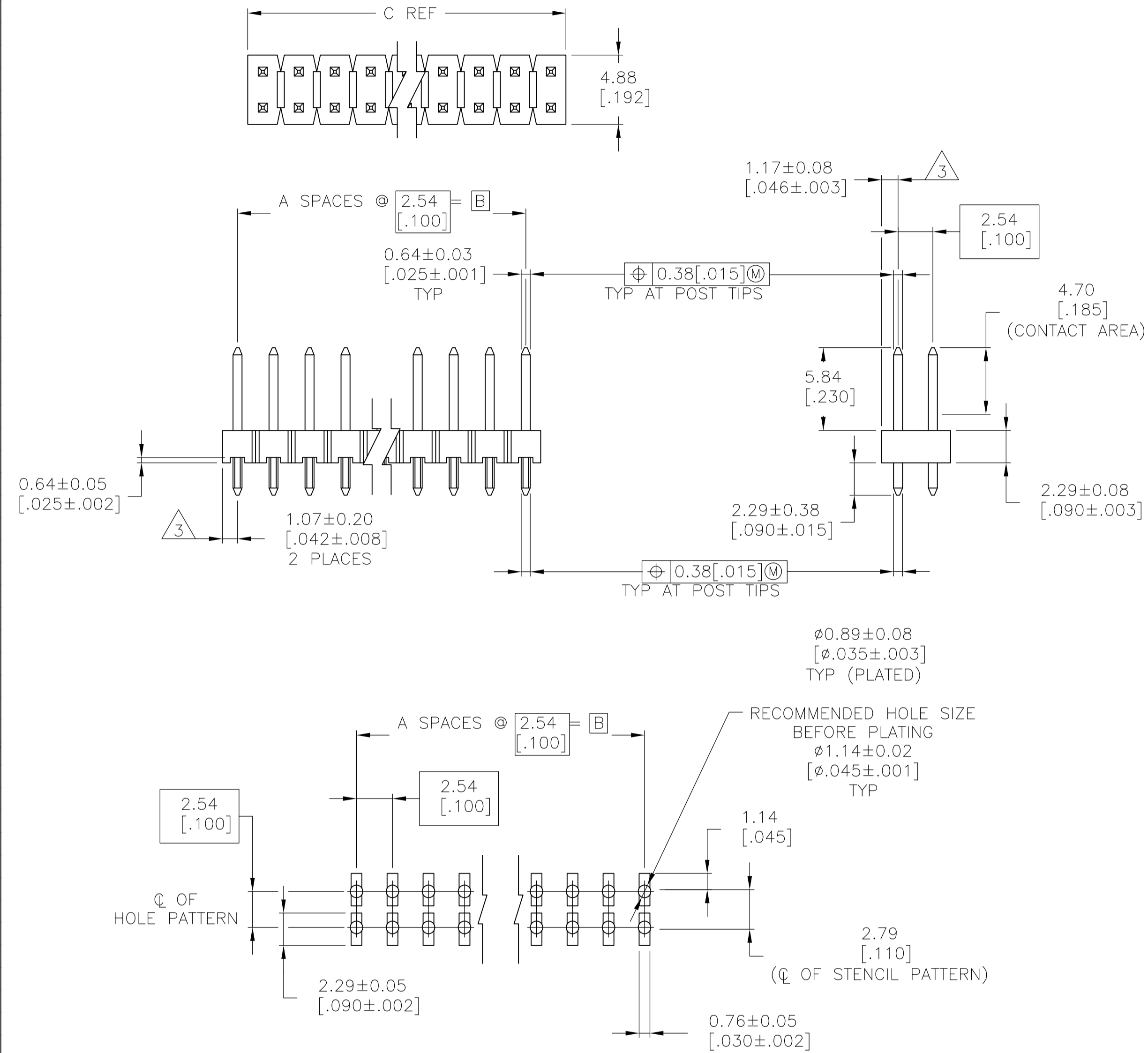
RECOMMENDED PC BOARD MOUNTING DIMENSIONS FOR .063[1.60] THICK PC BOARD AND .012[.305] STENCIL THICK
