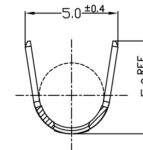
SECTION "C-C"
