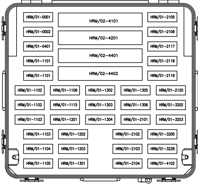
VIEW B-B ROTATED 90° COUNTER CLOCKWISE (FLYLEAF REMOVED FOR CLARITY)
