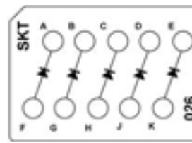
CTJ420E026 Five JANTX 1N5620 Diodes
