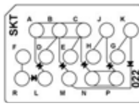
CTJ420E022 Six JANTX 1N5809 Diodes
