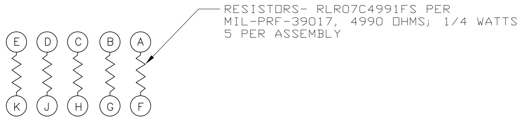
SCHEMATIC DIAGRAM
