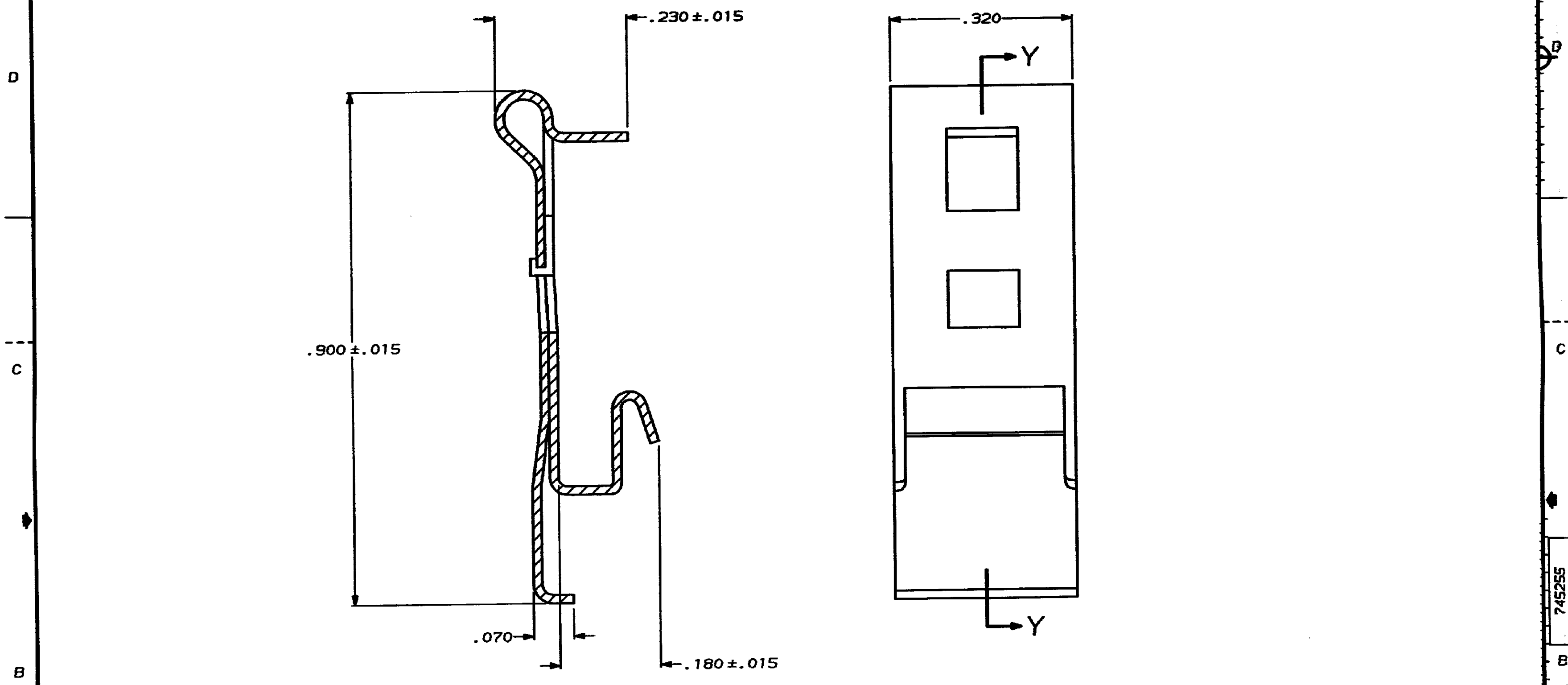
SECTION Y-Y
