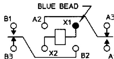
TERMINAL VIEW
