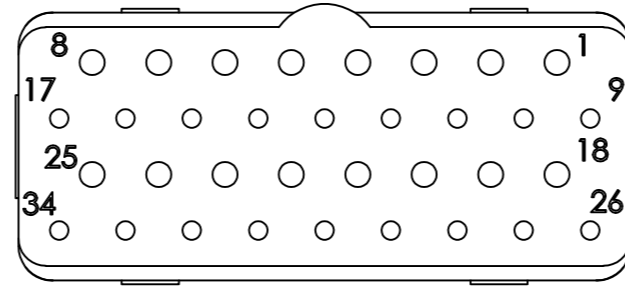
MATING FACE
