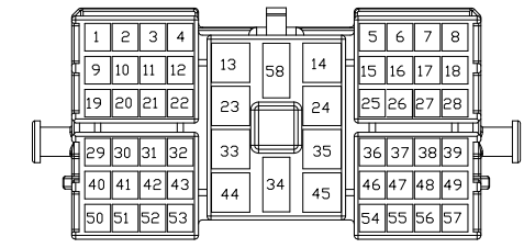
T300 BODY-IP CONN. FEMALE HOUSING ASS'Y
