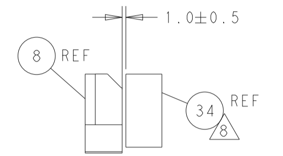
TERMINAL SUPPORT LOCATION FOR ALL SOCKET TERMINALS
