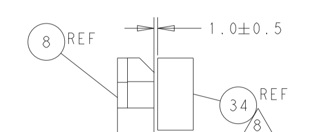
TERMINAL SUPPORT LOCATION FOR ALL SOCKET TERMINALS
