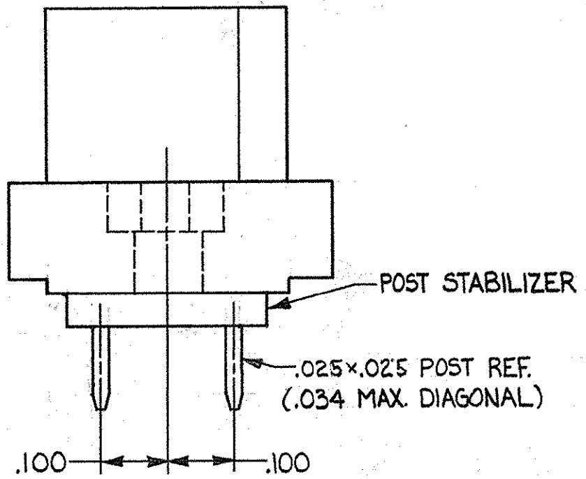
WRAP TYPE POST 3 HIGH CONTACT (-2, -4, -6, -8) ⑤ 2 ROW
