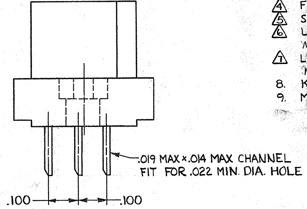
FLOW SOLDER POST CONTACT (-9, 1--1, 1--3, 1--5) 3 ROW
