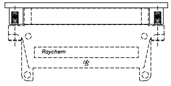
PLUG CONNECTOR
