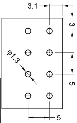
PCB Layout
