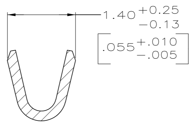
SECTION Y-Y WIRE BARREL SCALE 20:1
