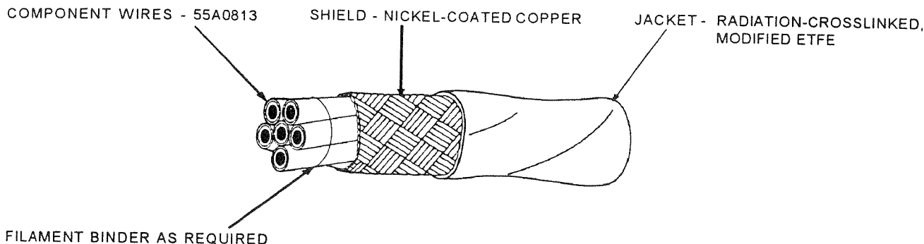
CABLE CONSTRUCTION DETAILS
