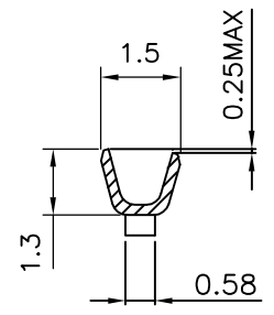
SEC B-B
