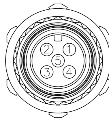
1838277-3 PIN ASSIGNMENTS FRONT VIEW
