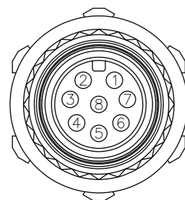
1838277-4 PIN ASSIGNMENTS FRONT VIEW
