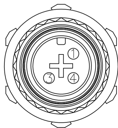
1838277-1 PIN ASSIGNMENTS FRONT VIEW
