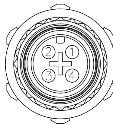
1838277-2 PIN ASSIGNMENTS FRONT VIEW
