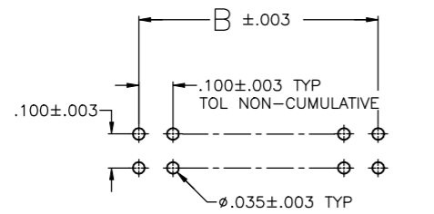
RECOMMENDED HOLE LAYOUT
