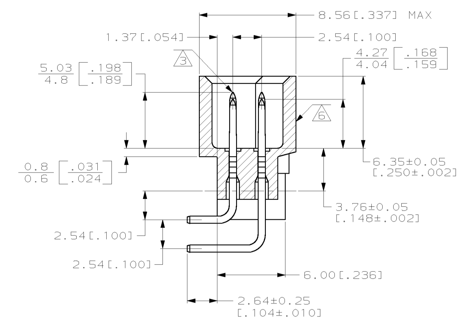
SECTION X-X
