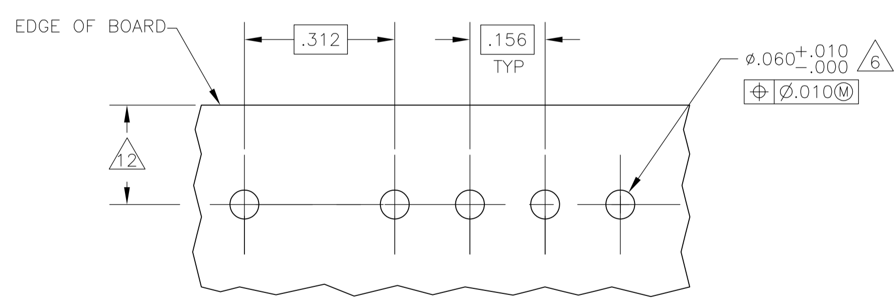
RECOMMENDED MOUNTING HOLE PATTERN FOR .063 THICK P.C.BOARD
