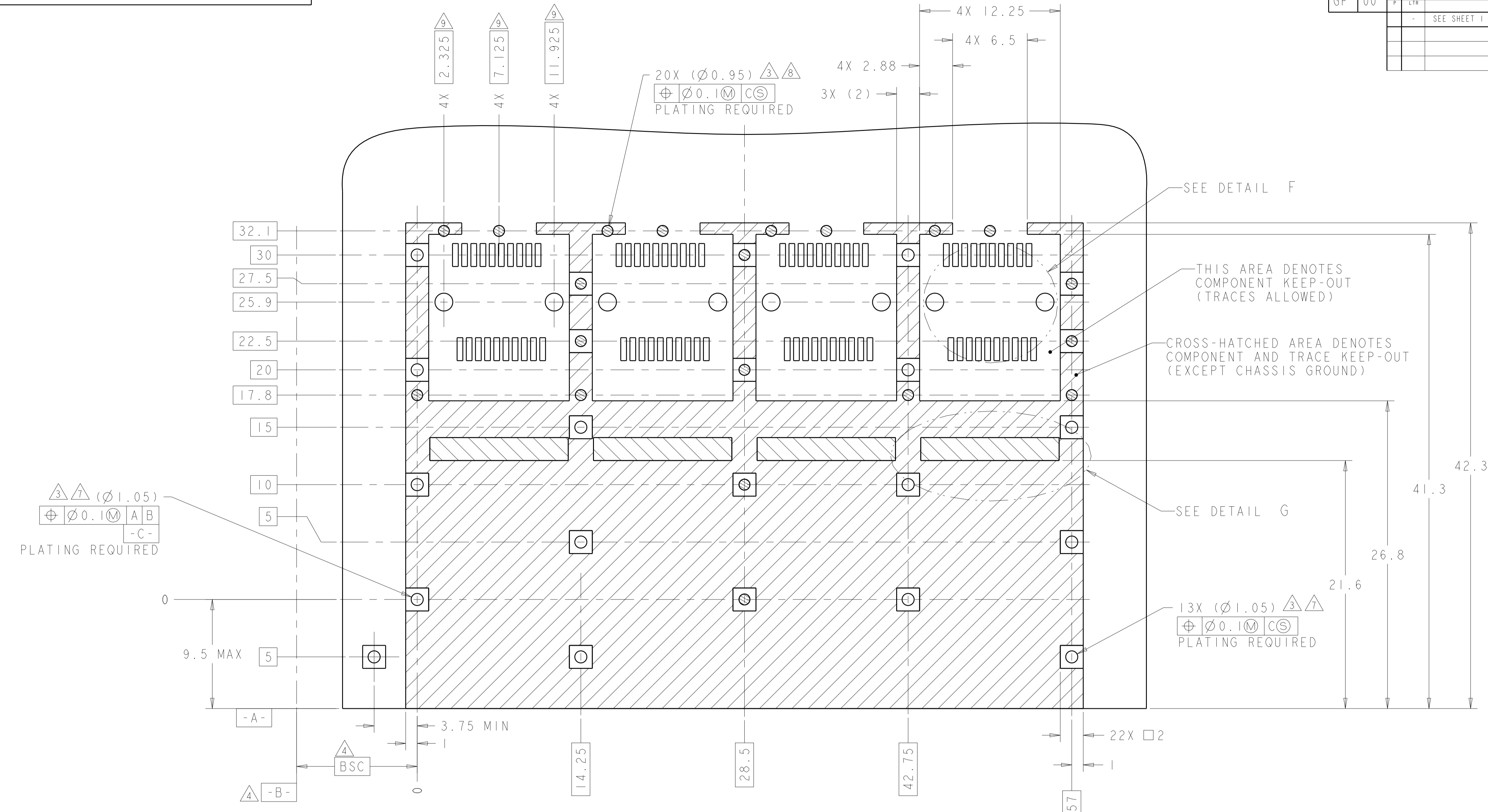
RECOMMEND PCB CONFIGURATION WITH KEEP-OUT AREAS FOR SINGLE SIDED APPLICATIONS SCALE 5:1
