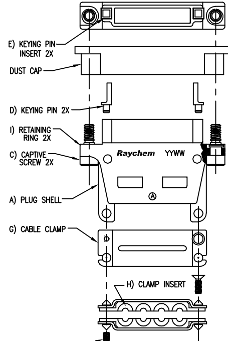
PLUG SHELL (4 CONTACTS - 12 AWG)
