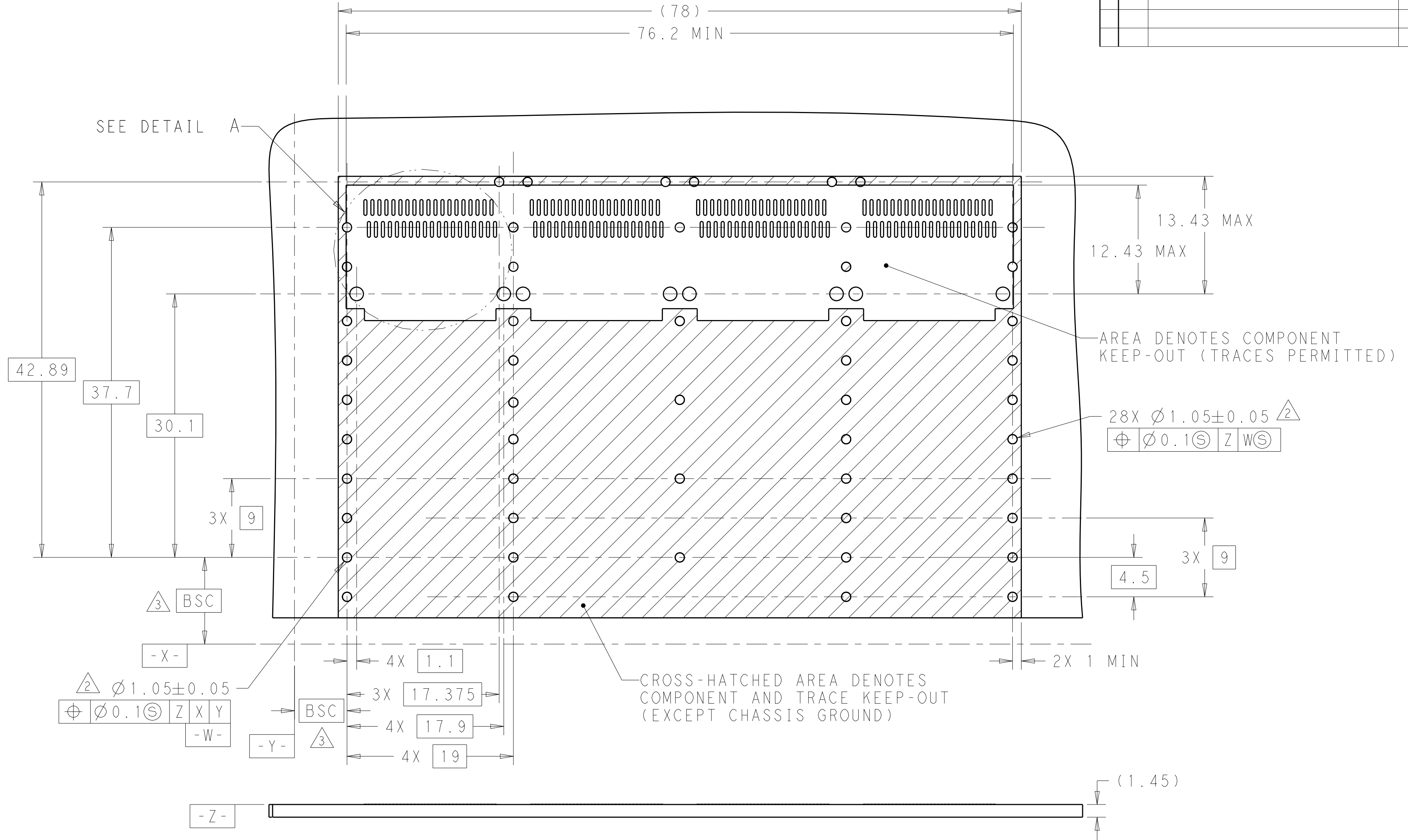
RECOMMENDED PCB LAYOUT SINGLE SIDE MOUNTED CONFIGURATION SCALE 3:1
