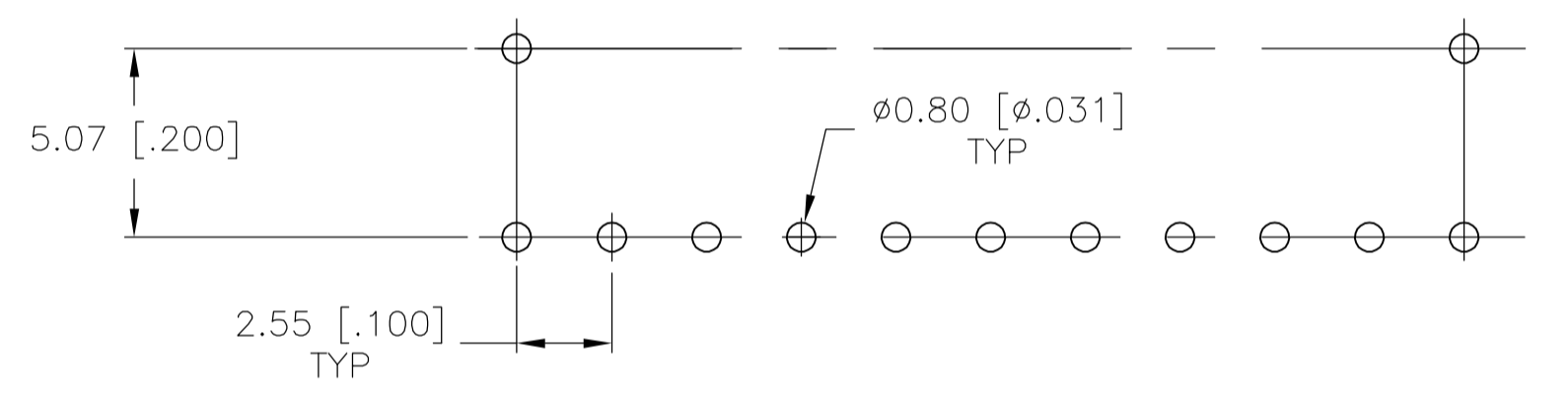
RECOMMENDED PCB HOLE LAYOUT
