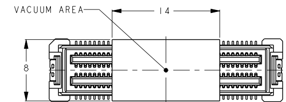
6376610-2:AS SHOWN WITH POLYIMIDE TAPE SCALE 3:1
