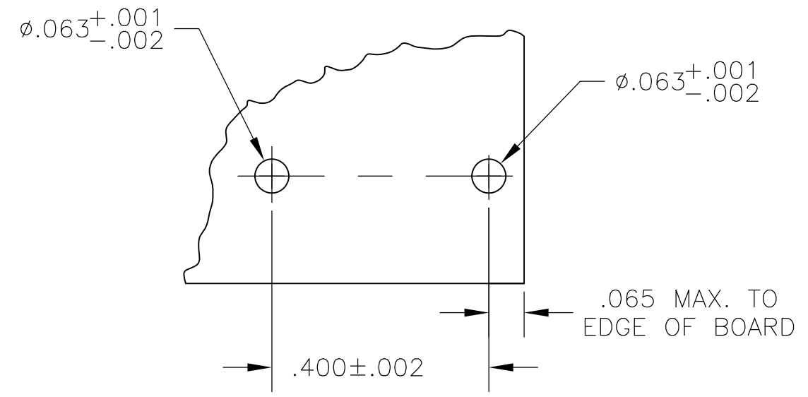
RECOMMENDED MOUNTING HOLES
