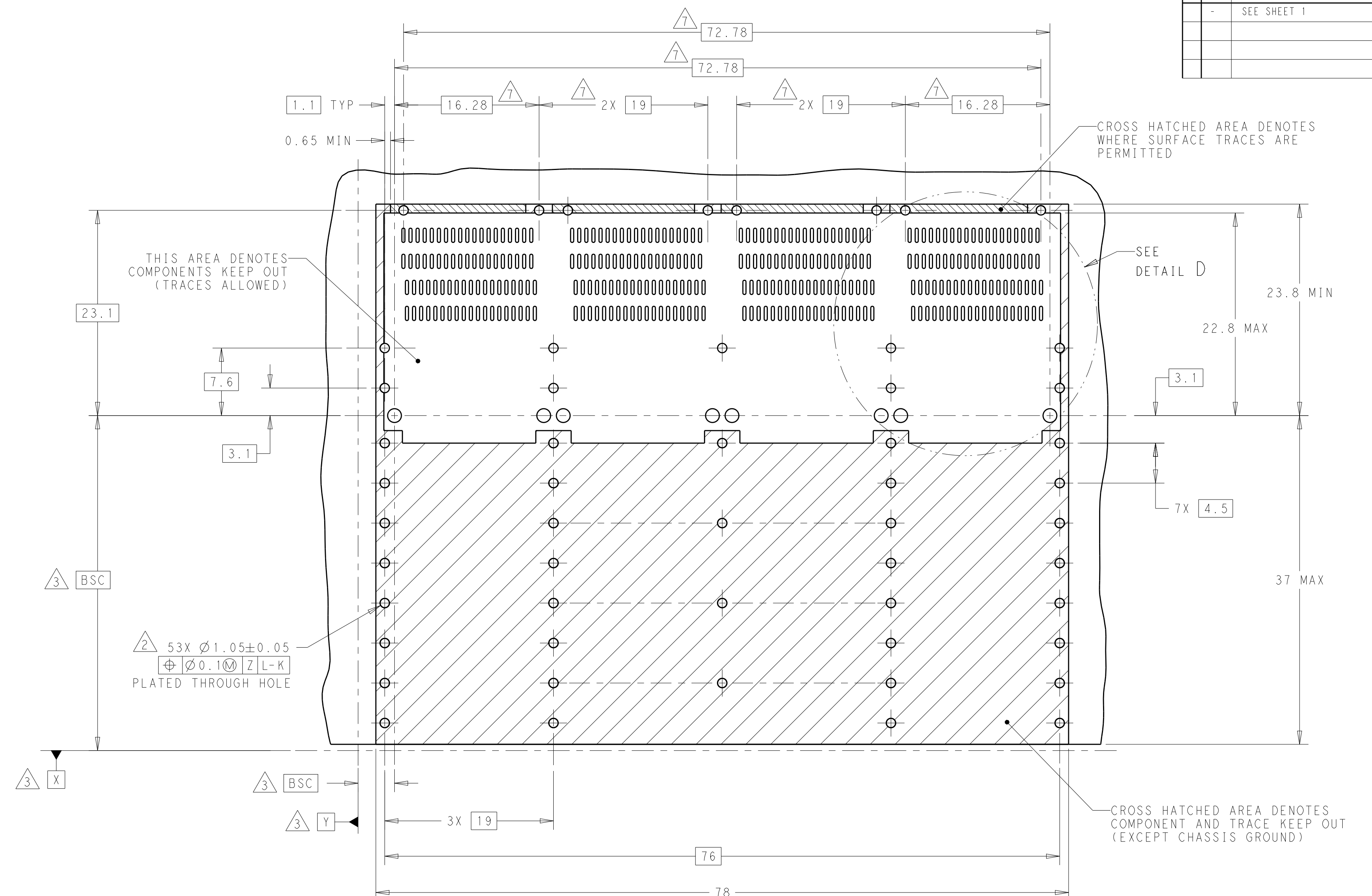
RECOMMENDED PCB LAYOUT BELLY TO BELLY SCALE 3:1
