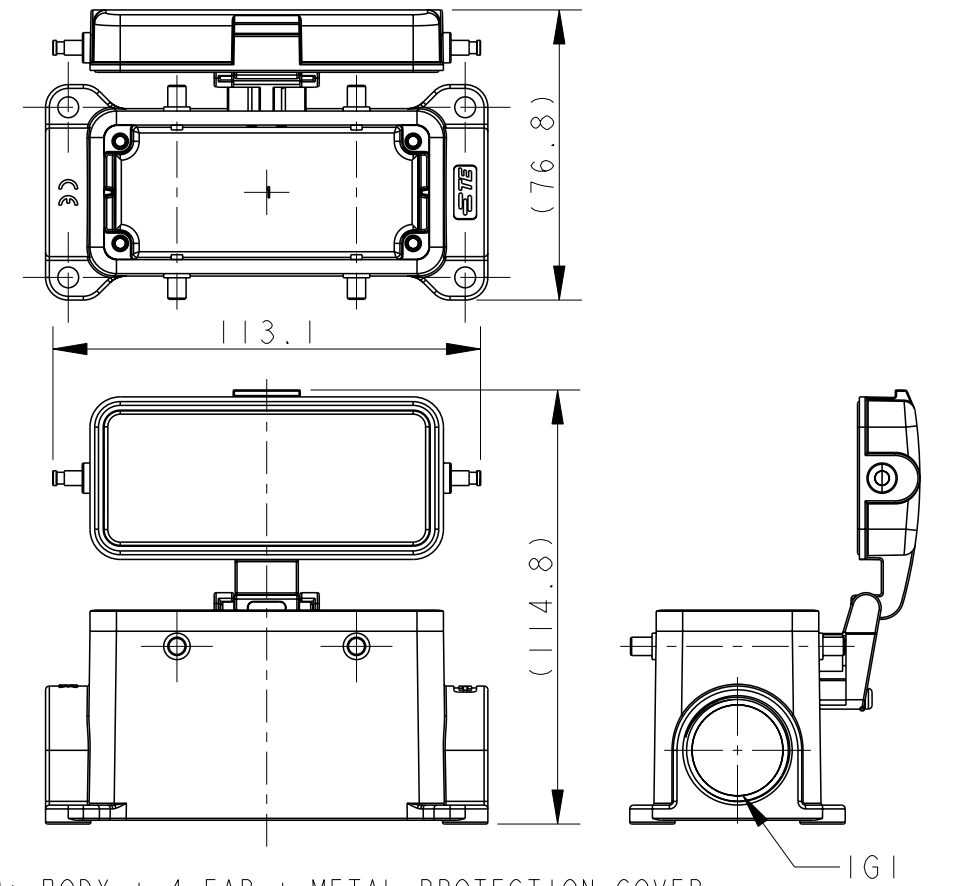
TYPE 2: BODY + 4 EAR + METAL PROTECTION COVER OTHER SPEC REFER TO TYPE 1
