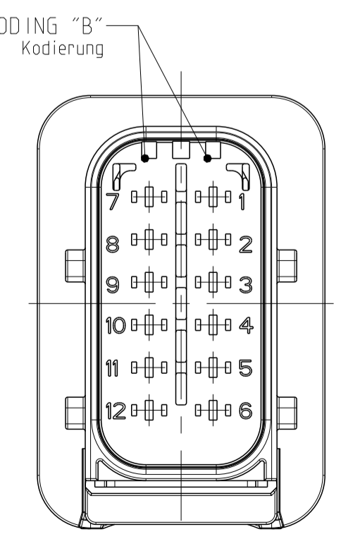
CODING "B" Kodierung PN: 2-1564414-1
