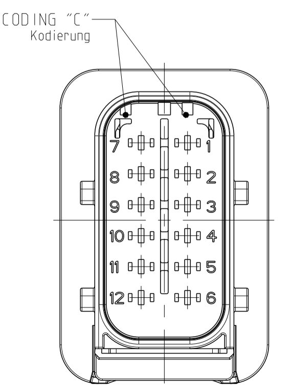
CODING "C" Kodierung PN: 3-1564414-1
