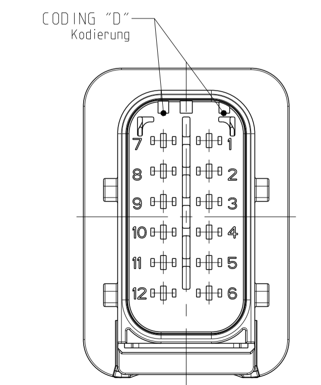
CODING "D" Kodierung PN: 4-1564414-1
