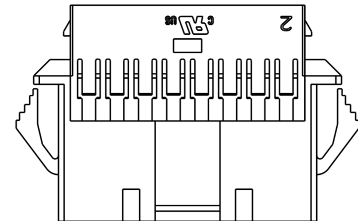
SINGLE LATCH DETAIL FOR 1-2324584-2 THRU 1-2324584-6
