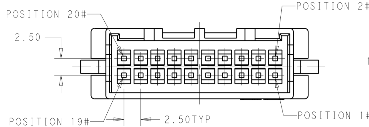
DUAL LATCH DETAIL FOR 1-2324584-8 THROUGH 4-2324584-0
