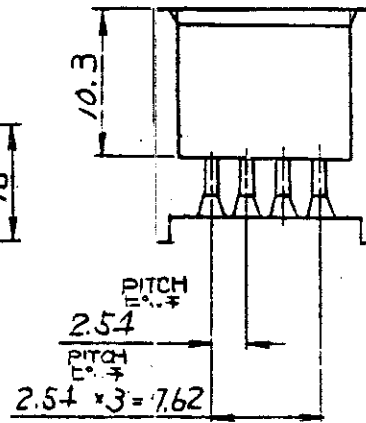
SECT "A-A"
