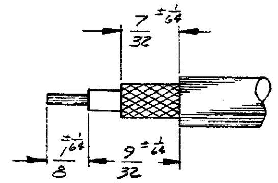
STRIP LENGTH
