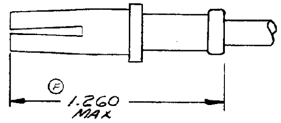
ASSEMBLED VIEW
