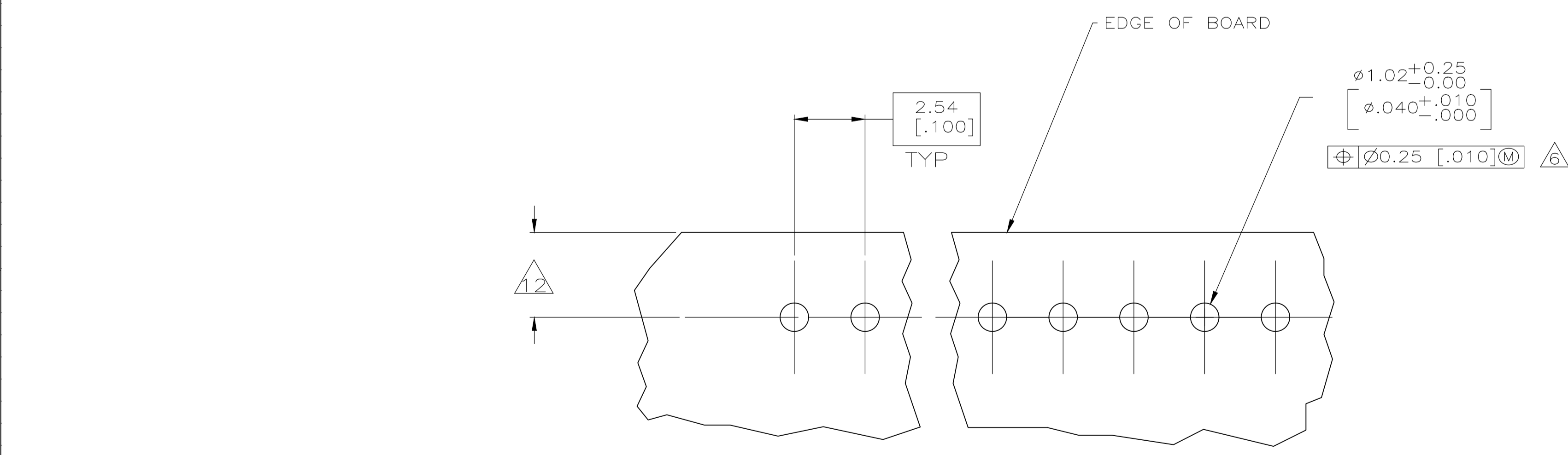
RECOMMENDED MOUNTING HOLE PATTERN FOR 1.60 [0.063] THICK P.C. BOARD
