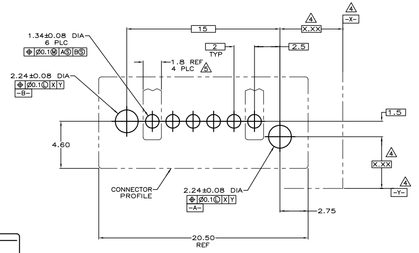
P.C. BOARD MOUNTING DIMENSIONS
