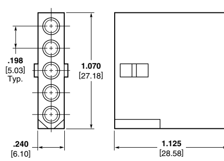
Receptacle (Free-Hanging)
