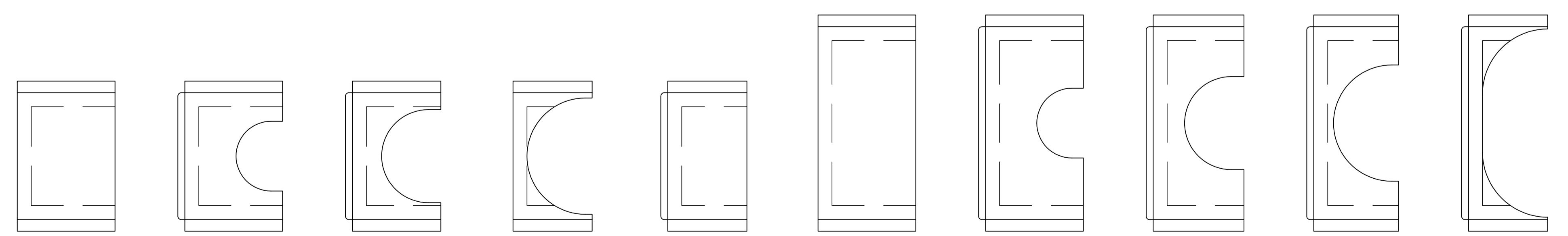
4-A .250 DIA CABLE REF 4-B .265 DIA CABLE REF 4-C .390 DIA CABLE REF 4-D .405 DIA CABLE REF 4-E BLANK GATE 4-F BLANK GATE 4-G .270 DIA CABLE REF 4-H .320 DIA CABLE REF 4-J .400 DIA CABLE REF 4-K .640 DIA CABLE REF
