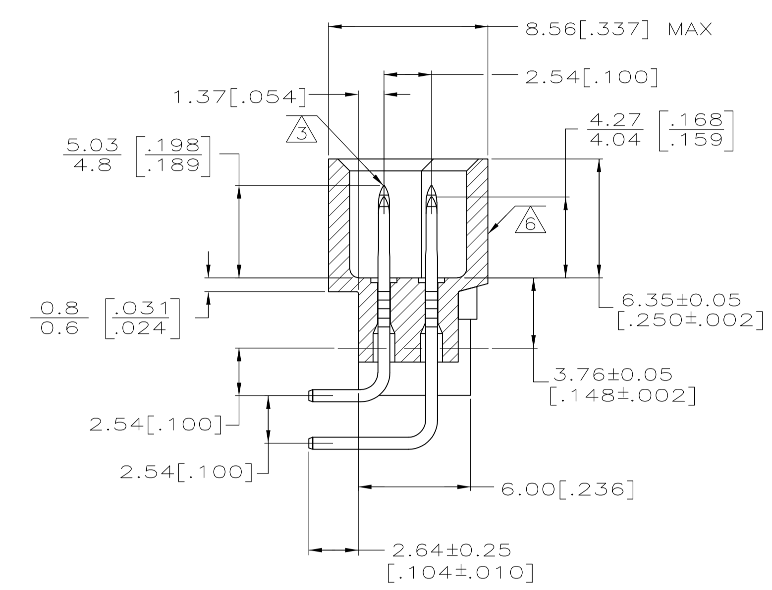
SECTION X-X
