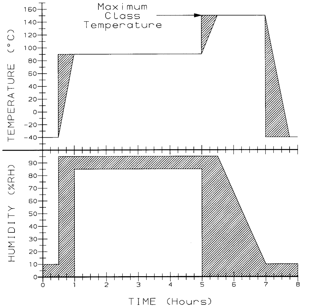
Figure 8 Humidity-Temperature Cycling Profile
