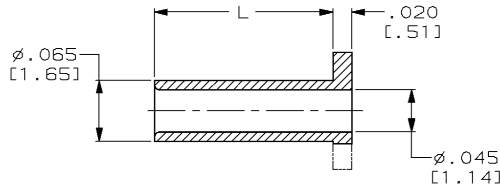
SECTION Z-Z
