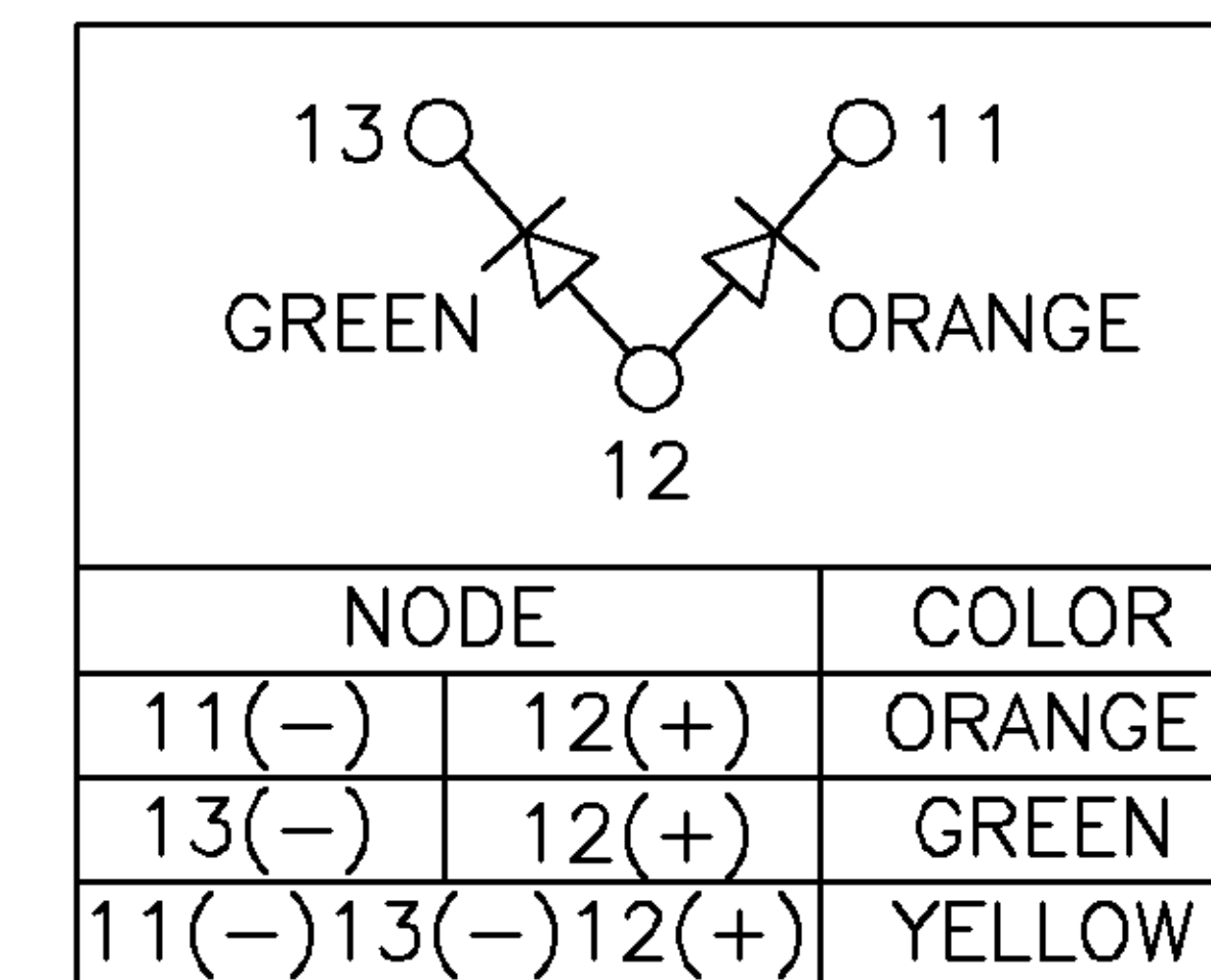
ELECTRICAL CIRCUIT
