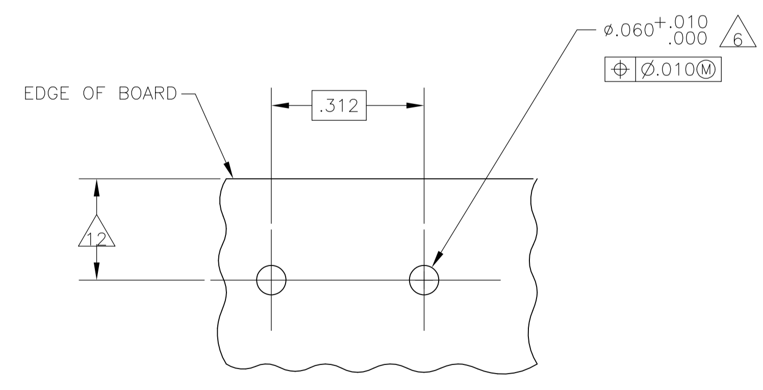
RECOMMENDED MOUNTING HOLE PATTERN FOR .063 THICK P.C. BOARD
