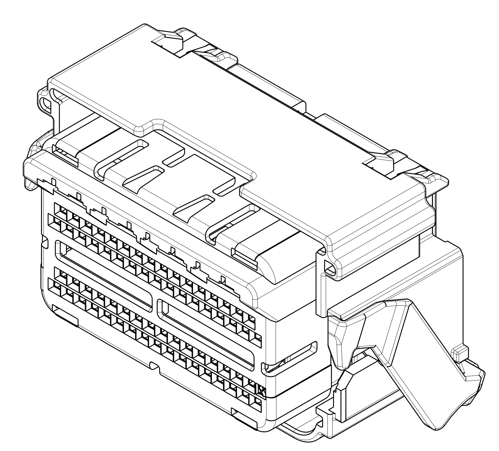
ISOMETRIC VIEWS
