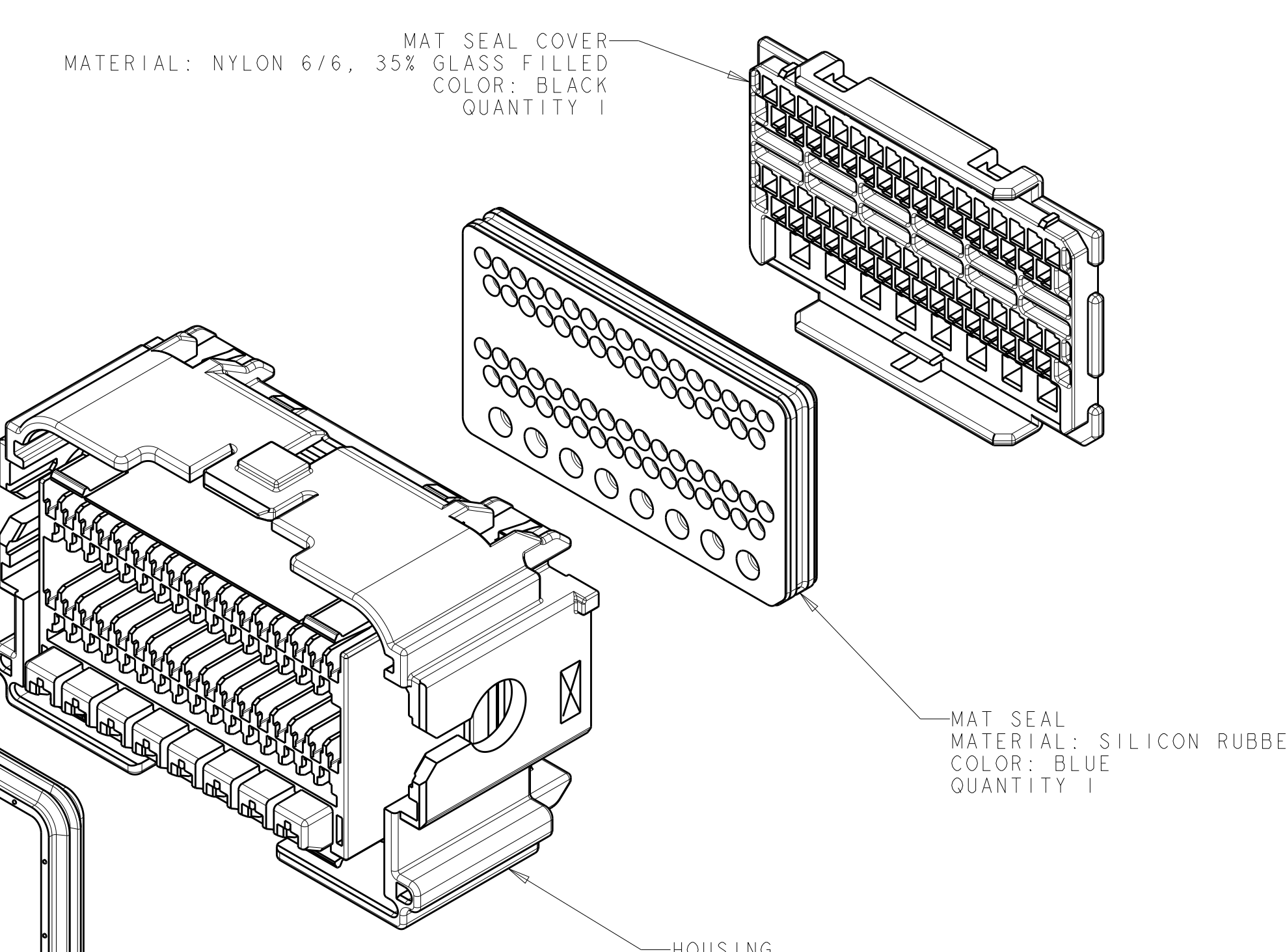
EXPLODED ISOMETRIC VIEW PART NUMBER: 776905-1 SHOWN FOR REFERENCE ONLY SCALE 2:1
