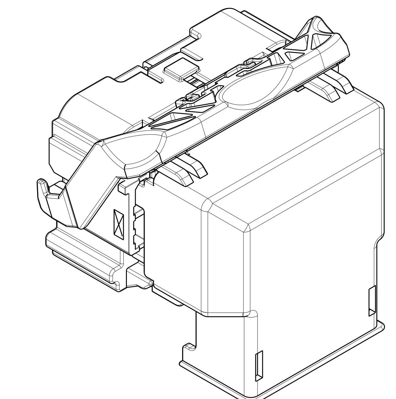
ISOMETRIC VIEW SHOWING THE OPTIONAL 90° EXIT WIRE GUIDE SCALE 2:1
